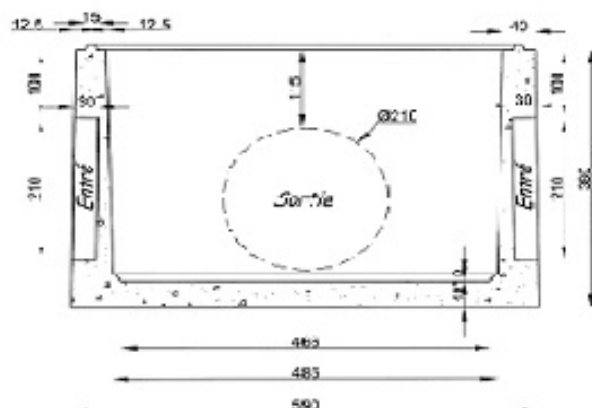
REGARD 500X500
